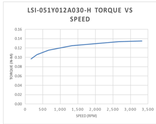
Example of typical use motor speed curve Higher speeds possible and is dependent on the applied voltage. Top speed may be limited mechanically. Please consult factory if higher speeds are required.
