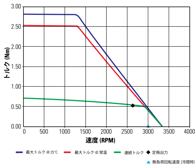
TBM(S)-6025-A 48 Vdc (6 step で計測)
