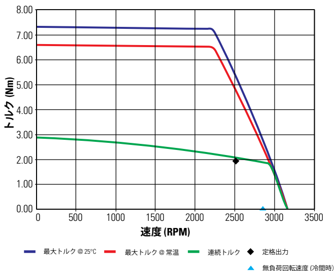
TBM(S)-12913-B 48 Vdc (6 step で計測)
