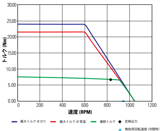
TBM(S)-12941-B 48 Vdc (6 step で計測)
