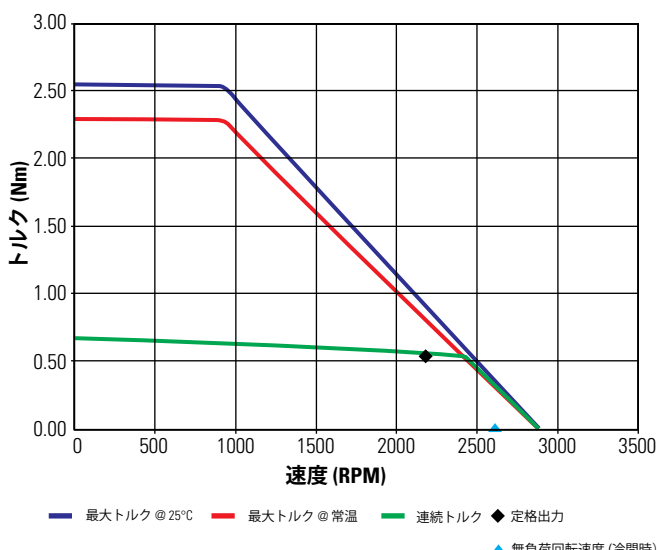
TBM(S)-6025-B 24 Vdc (6 step で計測)
