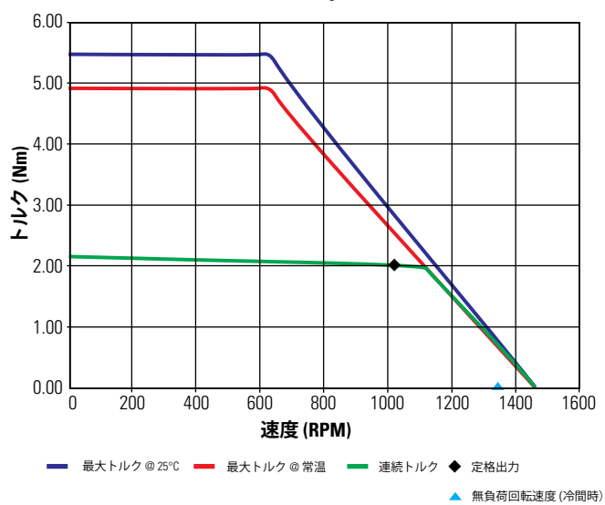
TBM(S)-7646-B 24Vdc (6 step で計測)
