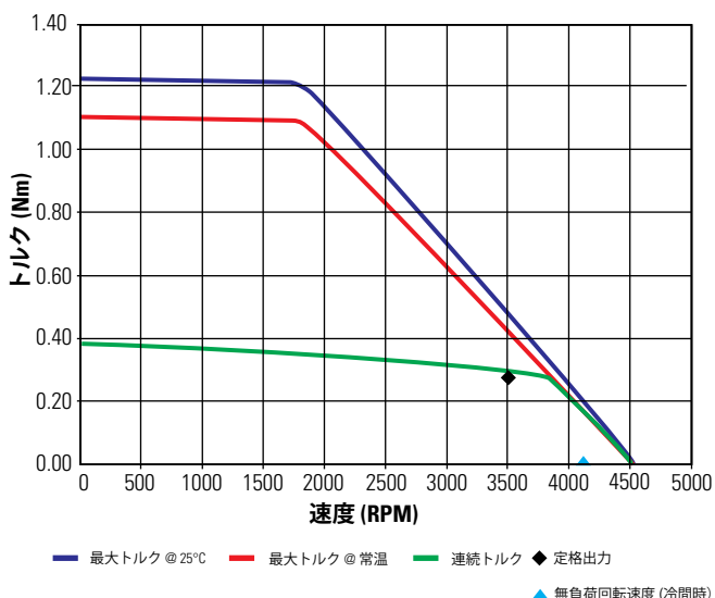
TBM(S)-6013-B 24 Vdc (6 step で計測)
