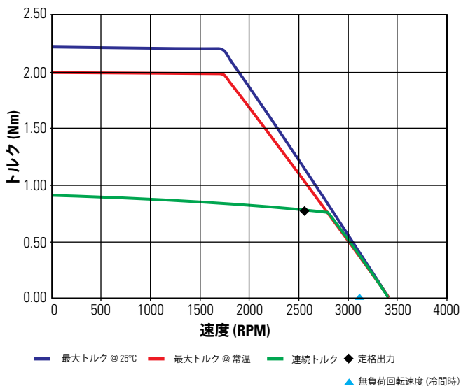
TBM(S)-7615-B 24 Vdc (6 step で計測)
