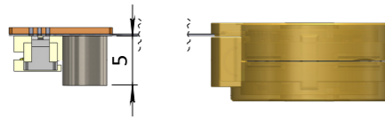
Bus bending radius 2 mm min.
